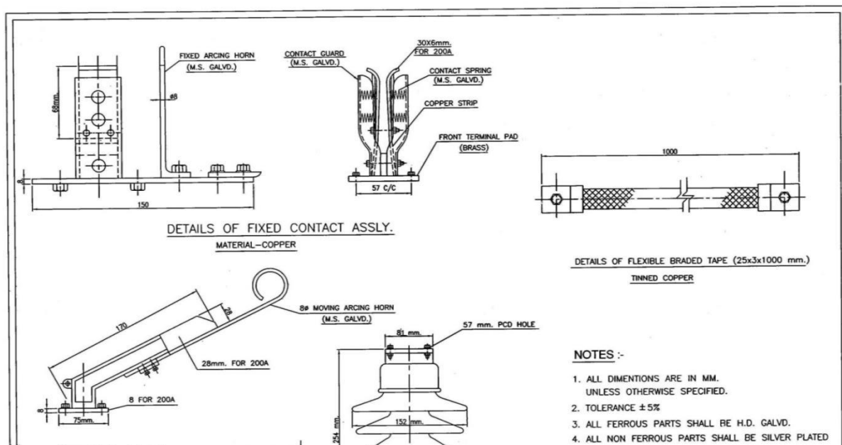
Figure-1, Rocking Type, 2 Post G.O.A.B.Switch
