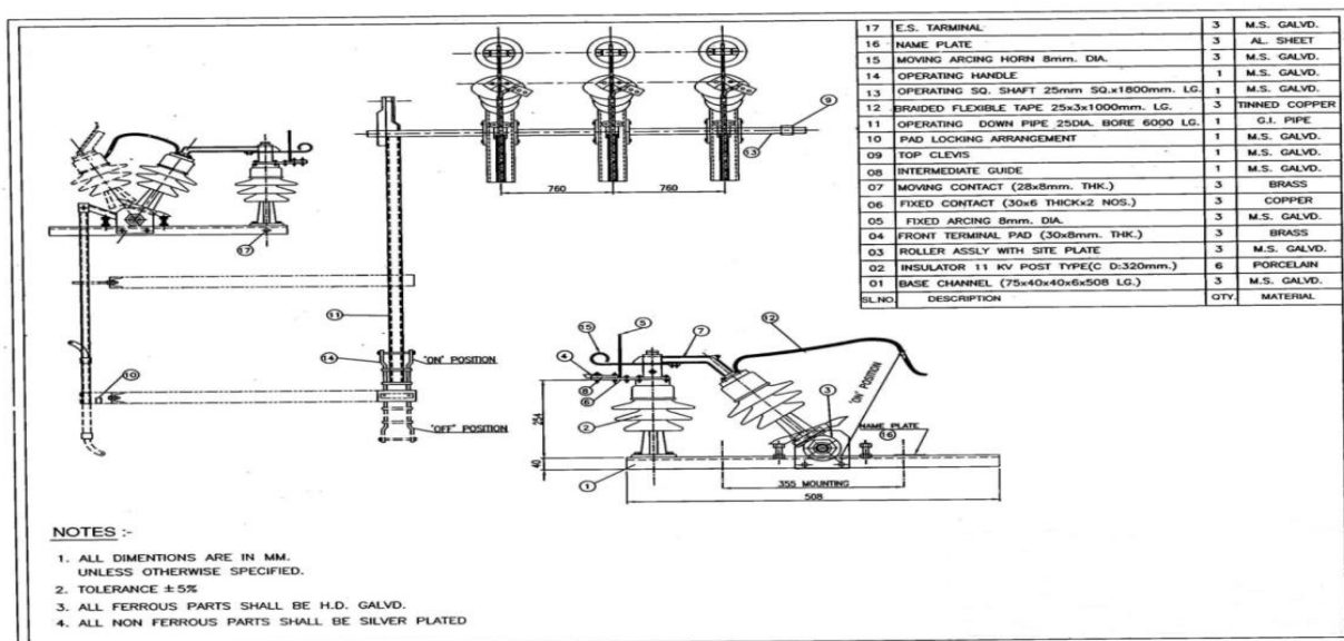
Figure-1, Rocking Type, 2 Post G.O.A.B.Switch
