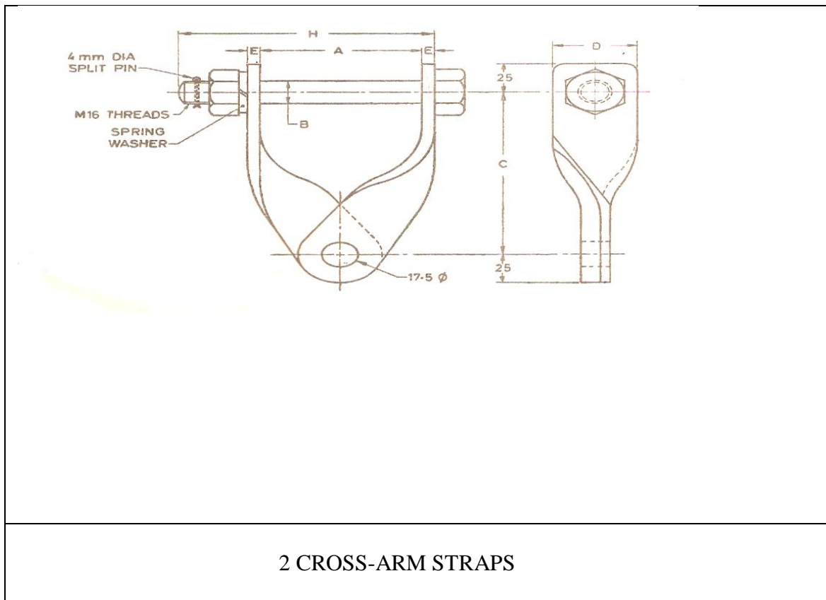
Fig. 1 SINGLE INSULATOR TENSION FITTING
