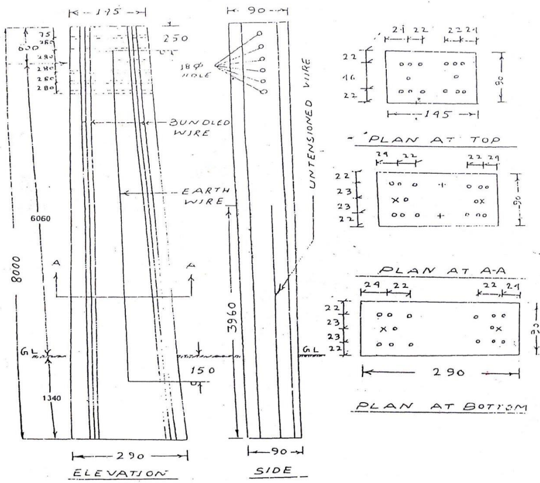
REINFORCEMENT DETAILS OF 8.0 M/200KG PRESTRESSED CONCRETE POLE
