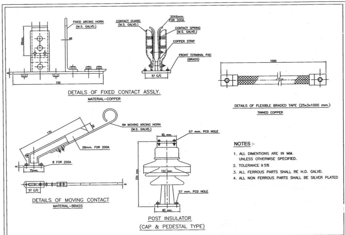
Figure-1, Rocking Type, 2 Post G.O.A.B.Switch
