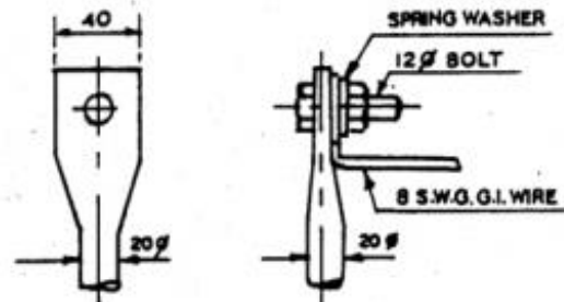
TYPICAL DETAIL OF CONNECTION FOR ROD EARTH
